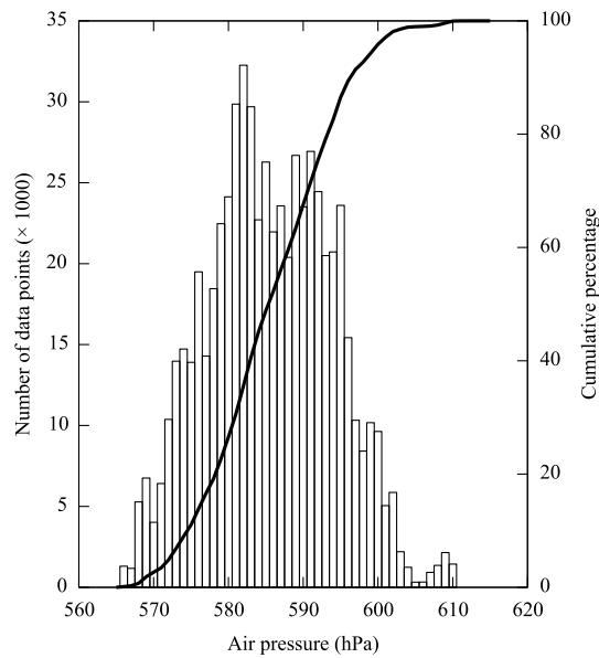
FIG. 20.—Air pressure histogram and cumulative distribution ( solid line ) during 2011.
