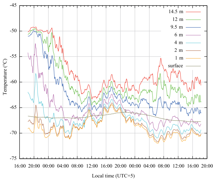
FIG. 8.—Temperatures at different heights between 2011 May 15 and 2011 May 17. A positive temperature gradient existed as low as 1 m and lasted for more than 2 days at all levels. This is indicative of very low atmospheric turbulence. See the electronic edition of the PASP for a color version of this figure.
