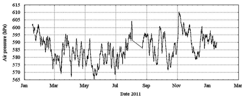
FIG. 19.—Air pressure during 2011. The raw data for the entire year are shown in this figure. Note that the barometric data should not be influenced by the collapse of the upper part of the mast in September.
