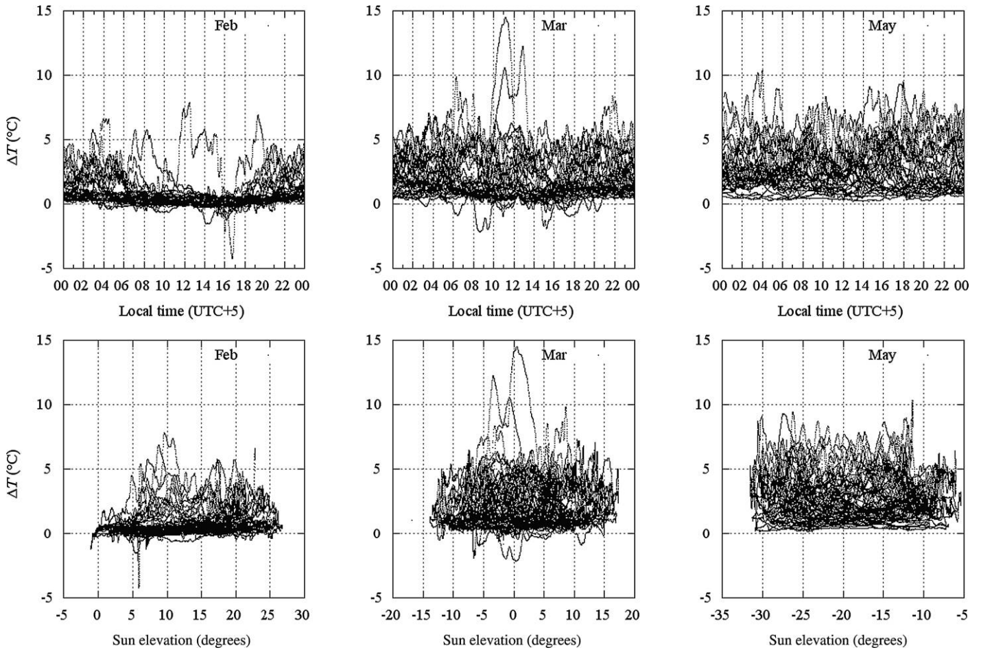
FIG. 12.—Temperature difference between 6 m and 4 m folded into a day during February, March, and May (top) and the same temperature difference vs. solar elevation (bottom).
