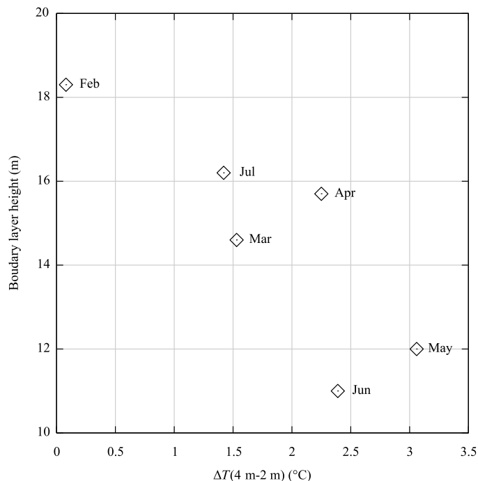
FIG. 22.—Monthly median boundary layer height during 2009 (Bonner et al. 2010) vs. the monthly median temperature difference between heights of 2 m and 4 m during 2011.
