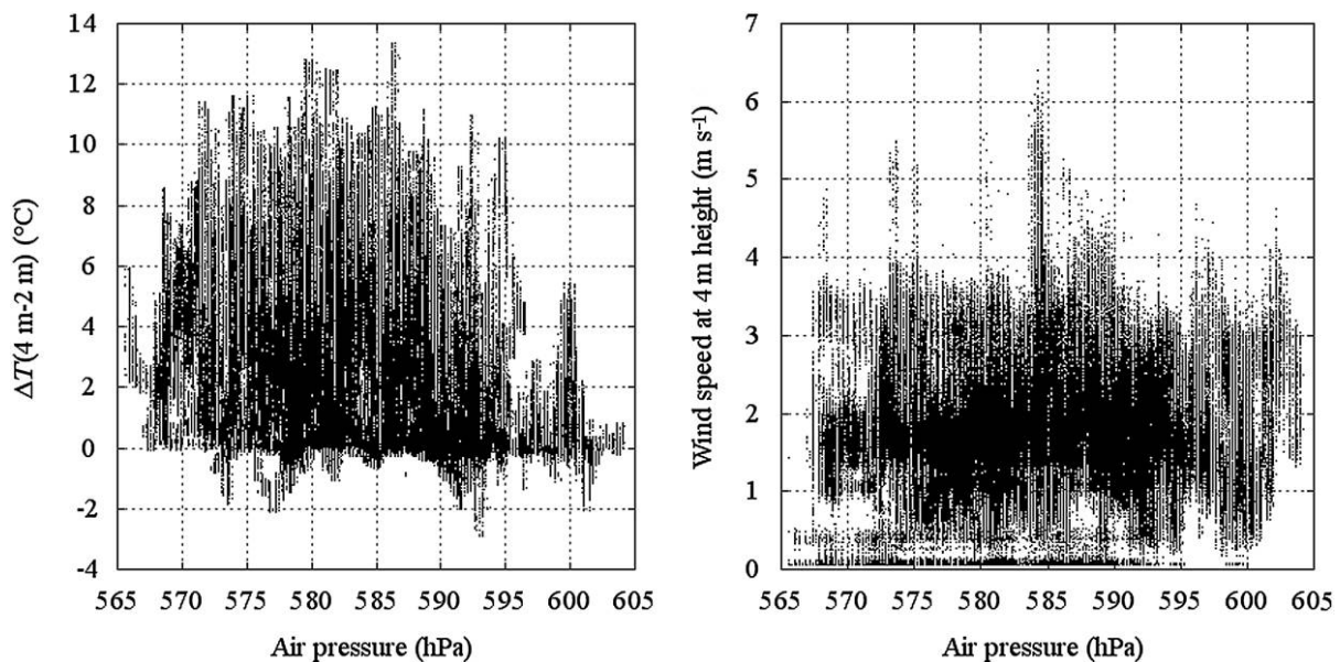
FIG. 21.—Temperature difference between the 2 m and 4 m heights ( left panel ) and wind speed at 4 m ( right panel ) vs. air pressure during 2011.
