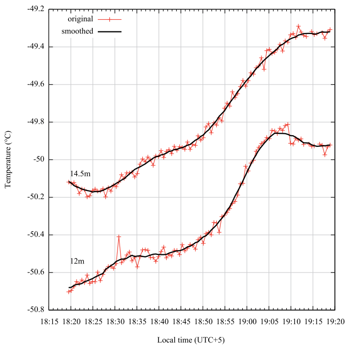
FIG. 4.—Example of temperature data smoothing for the 14.5 m and 12 m sensors for a 1 hr period on 2011 May 15. Note that the reproducibility of individual measurements on these timescales is much better than the absolute sensor accuracy of 0.32^{\circ}\text{C} . See the electronic edition of the PASP for a color version of this figure.
