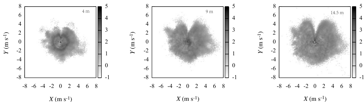
FIG. 15.—Wind rose density at three heights during 2011. North is up. The gaps are caused by the weather mast, which blocked the wind from the north direction. The gray scale is the logarithm of the number of data points per pixel. The obvious darker ring in the 4 m plot corresponds to the dominant wind speed, around about 1.7\text{ m s}^{-1} (see Fig. 14), of random directions. Similar patterns also exist in the other two plots, but are not as obvious.
