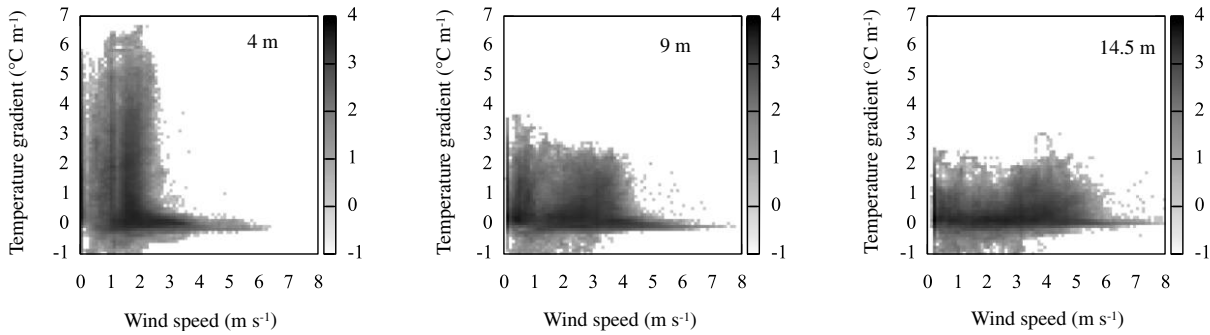
FIG. 18.—Wind speed against temperature gradient at the corresponding height. The gray scale is the logarithm of the number of data points per pixel. The vertical structures in the plots correspond to the real distribution of the data points in Fig. 14.
