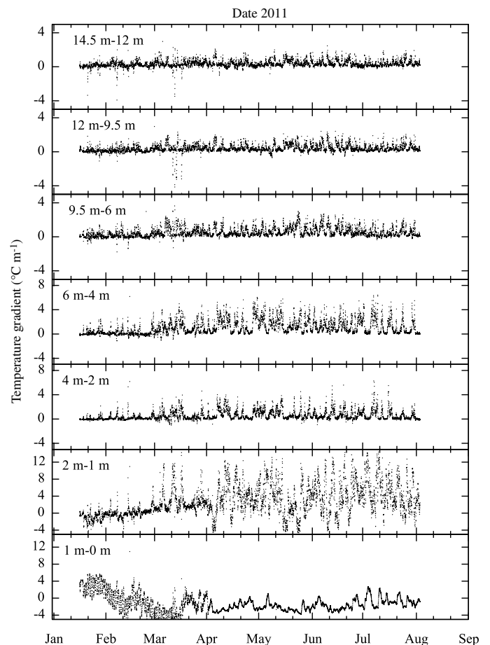
FIG. 9.—Temperature gradient between 2011 January and August at all levels. The temperature gradients were calculated from the smoothed data (see § 2). And, the data points were down-sampled by 100 for clarity.
