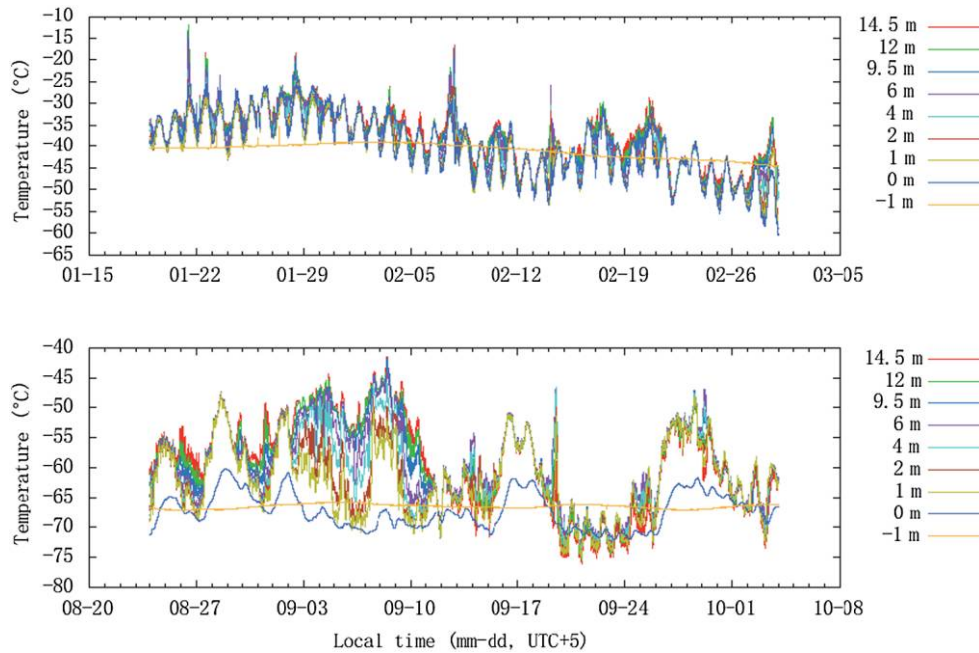
FIG. 3.—Temperatures recorded during the first 40 days of KL-AWS operation ( top panel ) in 2011 and 40 days following a restart of KL-AWS on 2011 August 23 ( bottom panel ). The changes in the temperature distribution after 2011 September 16 are believed to have been caused by the collapse of the upper part of the mast. This figure shows smoothed data (see § 2). See the electronic edition of the PASP for a color version of this figure.
