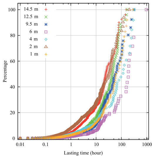
FIG. 13.—Cumulative distributions of the duration of the temperature inversion (defined as a positive temperature difference larger than 0.14° C) for all heights. See the electronic edition of the PASP for a color version of this figure.
