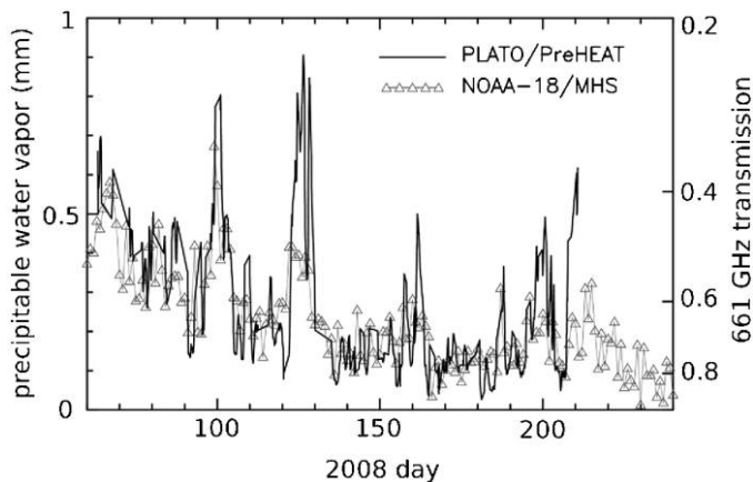
FIG. 1.—Overlay of the measured Pre-HEAT 661 GHz transmission ( solid line ) atop the 183 GHz microwave soundings ( triangles ), converted to 661 GHz equivalent, from the MHS instrument on NOAA-18 during 5 months of 2008. The left axis shows the precipitable water vapor corresponding to the observed transmissions. See the electronic edition of the PASP for a color version of this figure.
